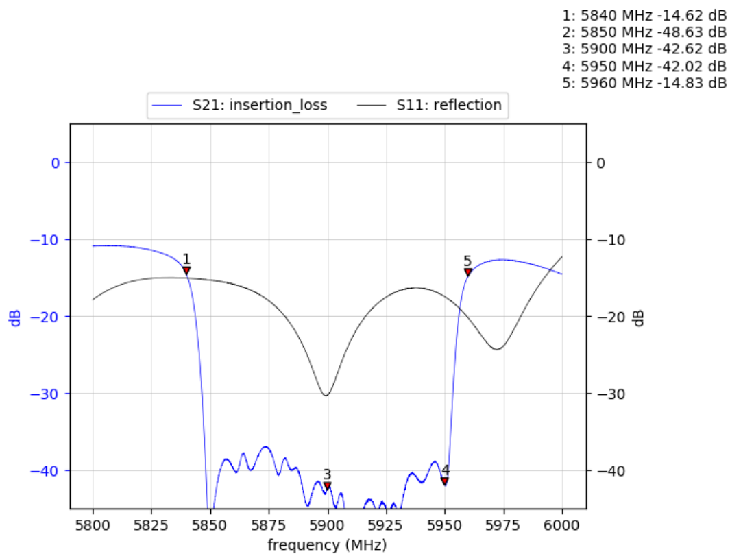
Example of 100 MHz band reject measurement
