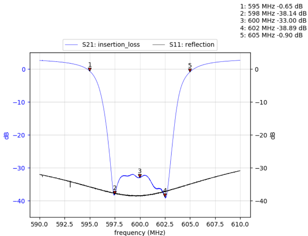
Example of 5 MHz band reject measurement
